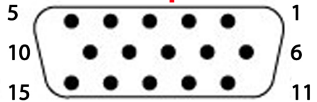
Female Plug Front View
