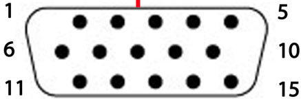
Male Plug Front View
